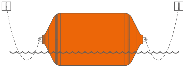
Mounting directly to concrete promotes wear
