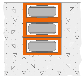
TRIPLE WHEEL
