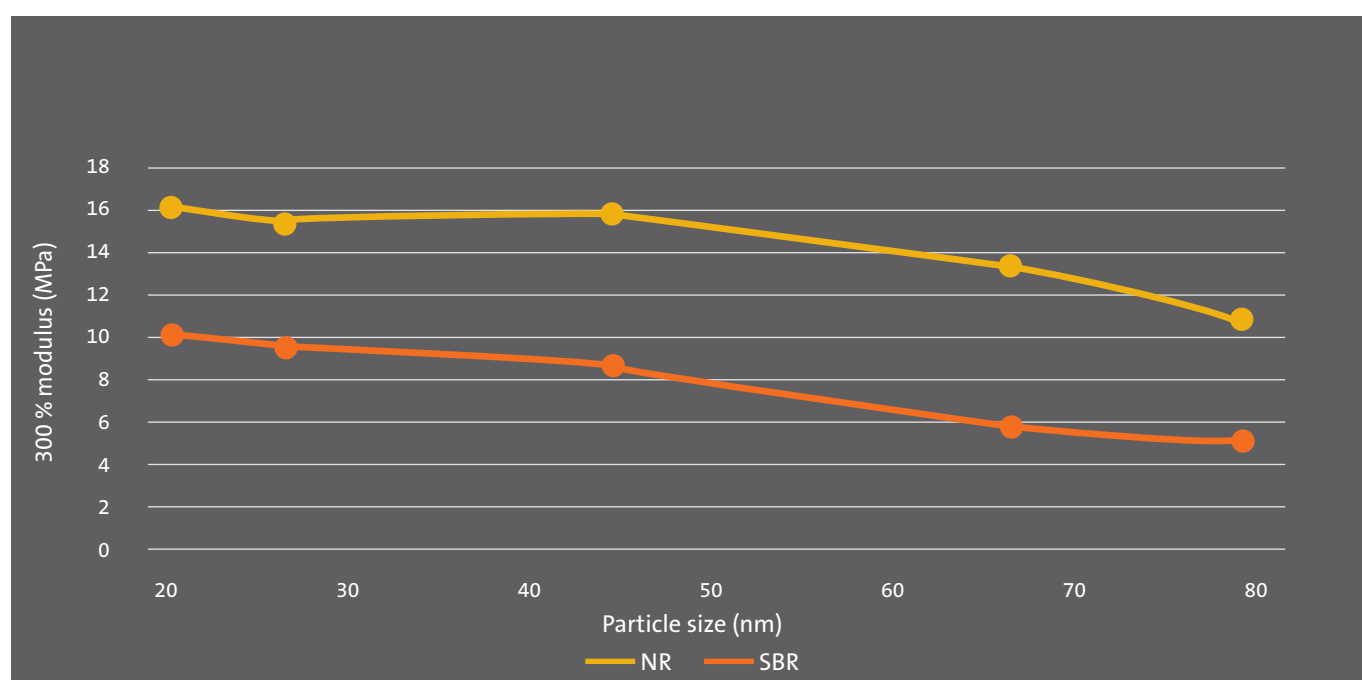
Figure 2: Modulus vs. particle size of CB (CB 33 %)
