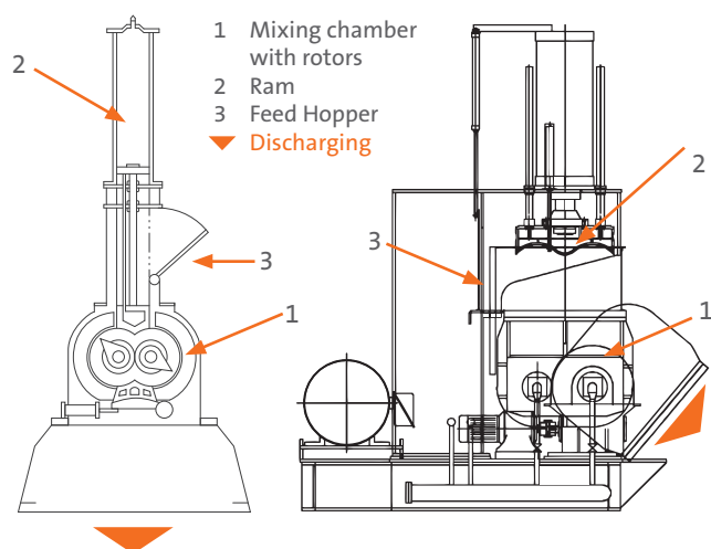
Drawing of a Banbury mixer
